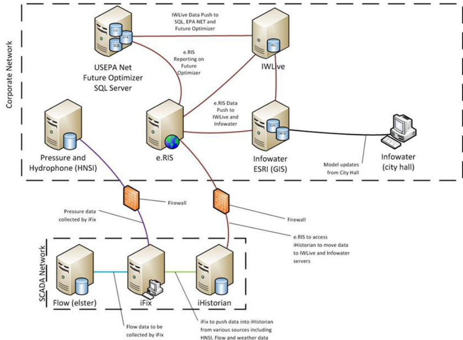
City of Guelph Waterworks Implementation of IWLIVE Data Flow Diagram
